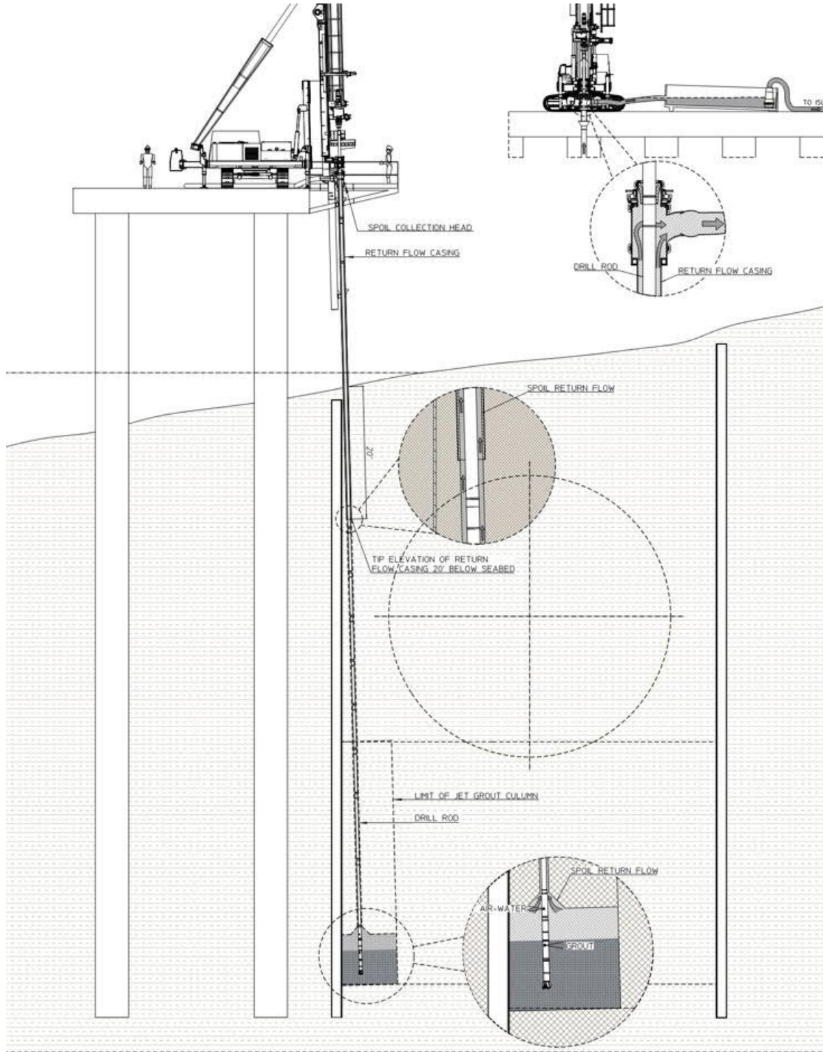
Figure L-6: Jet Grouting from Trestle Bridge Diagram
