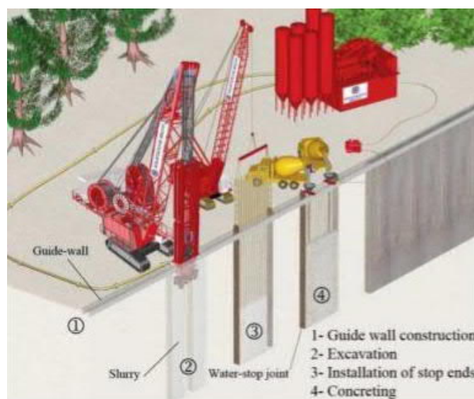
Figure L-7: Schematic of Slurry Wall Construction
