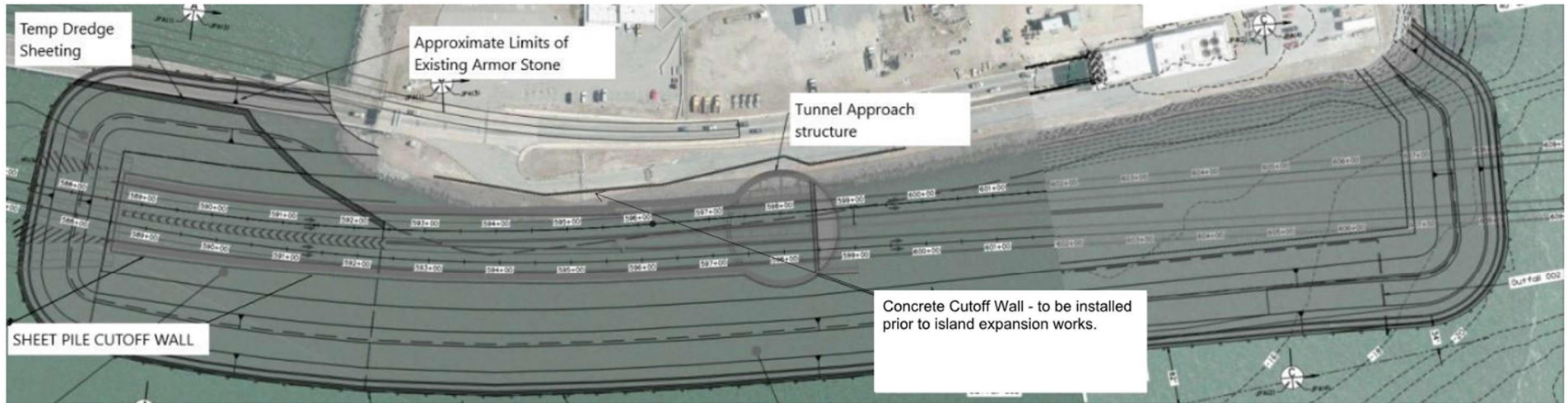
Figure L-8: North Island Expansion Proposed Sheet Pile Wall
