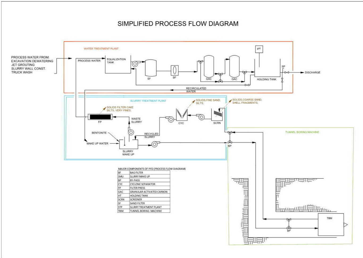
Figure L-13: Separation and Treatment Flow Diagram
