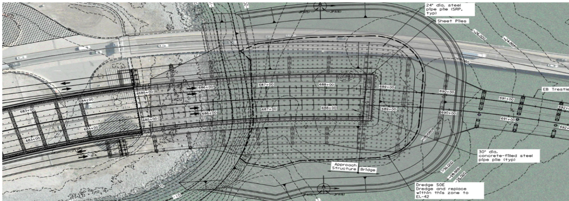
Figure L-9: South Island Expansion Proposed Sheet Pile Wall and Piles
