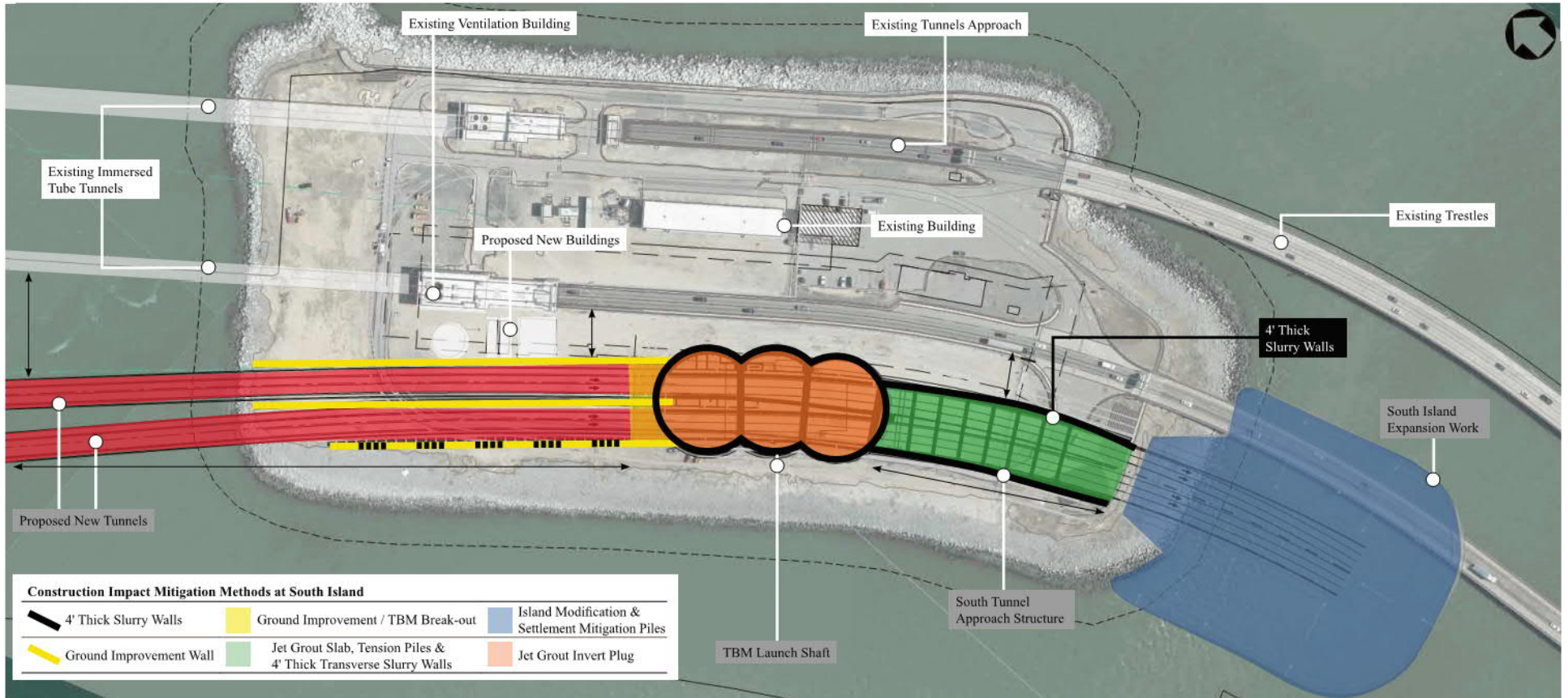
Figure L-4: South Island Layout
