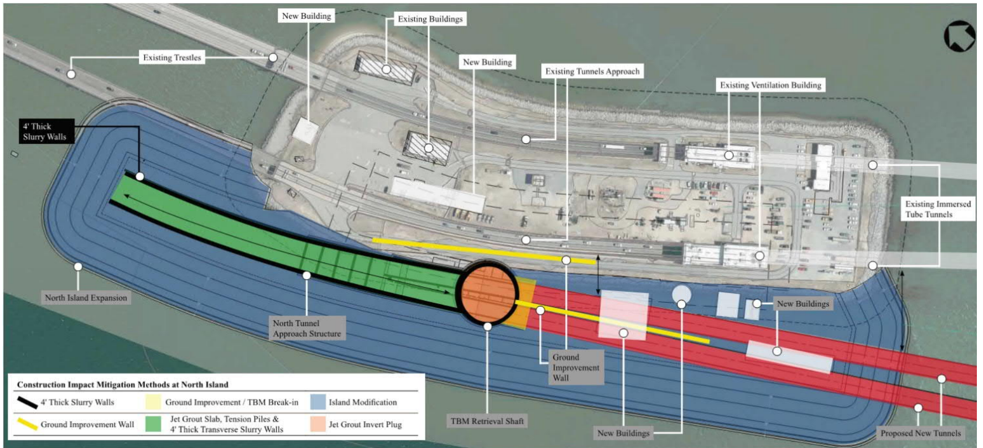
Figure L-3: North Island Layout
