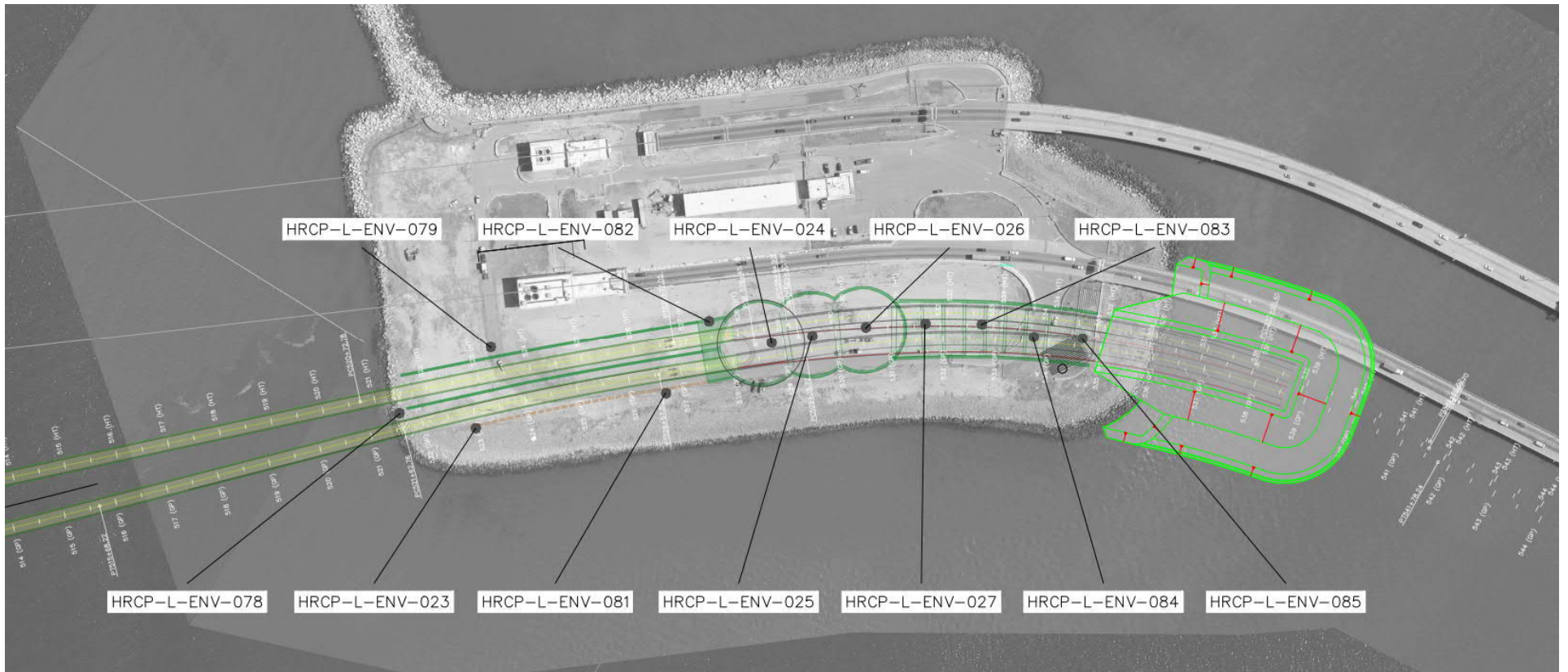
Figure L-12: Location of Environmental Borings on South Island
