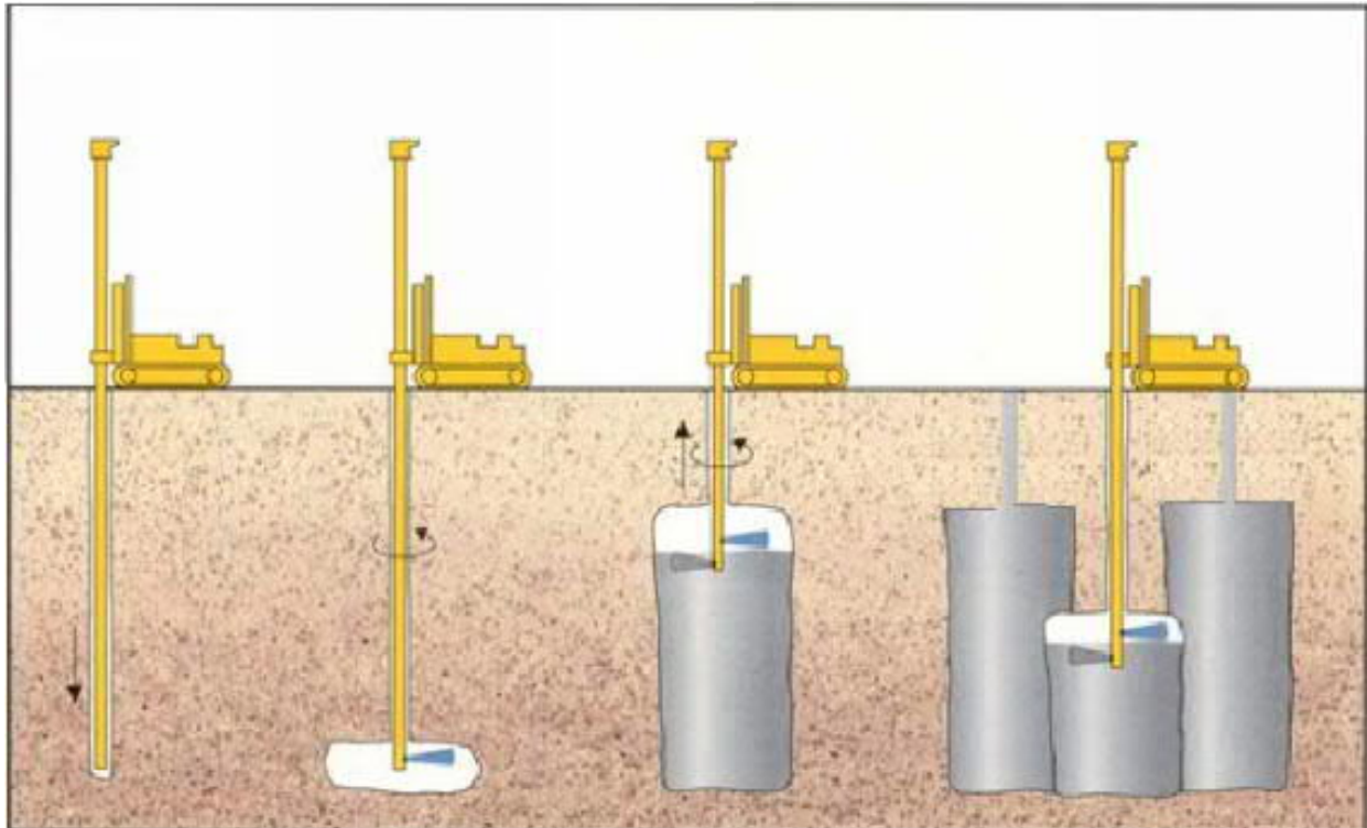
Figure L-5: Schematic of Jet Grouting Process
