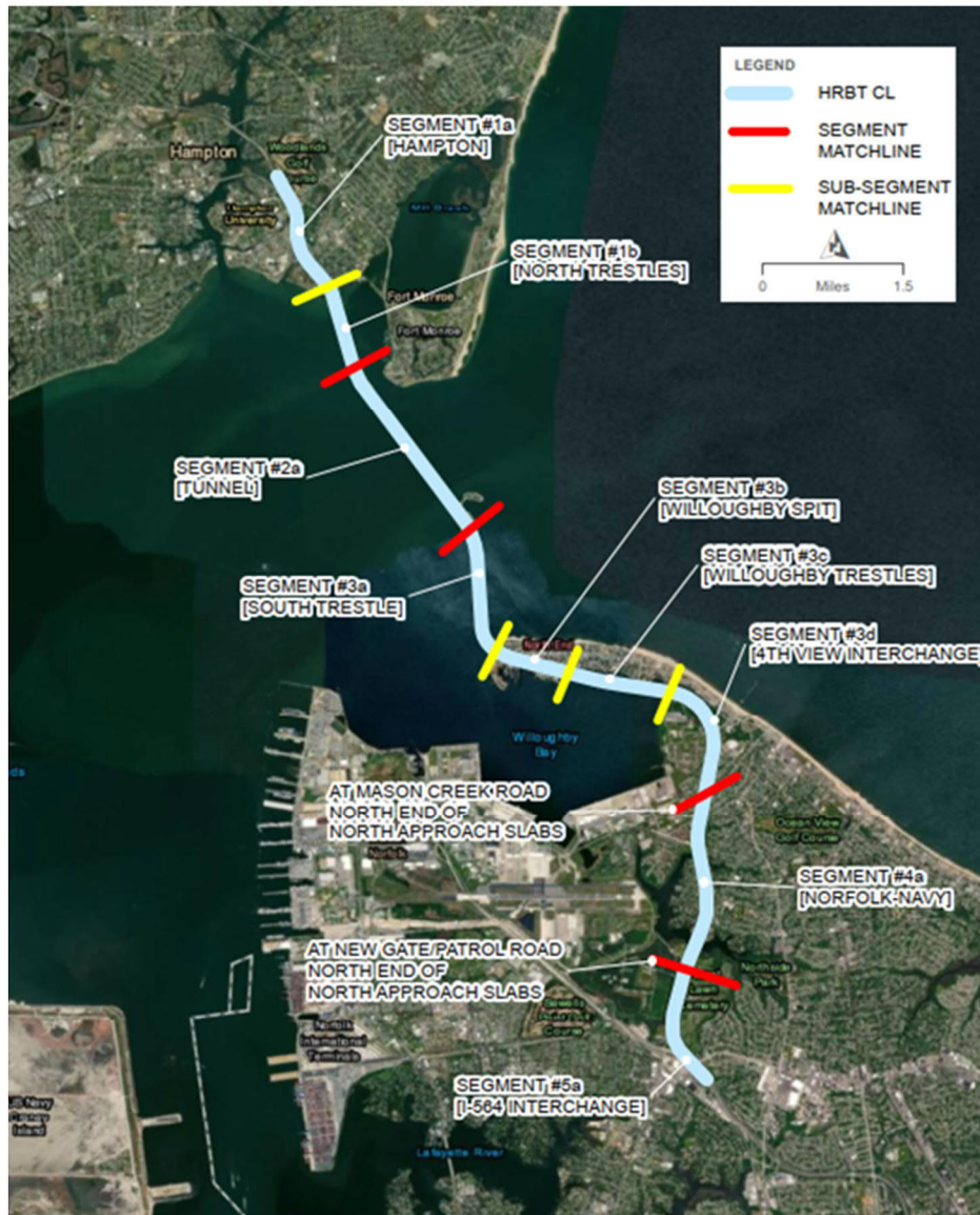
Figure L-2: HRBT Design Segments and Key Map
